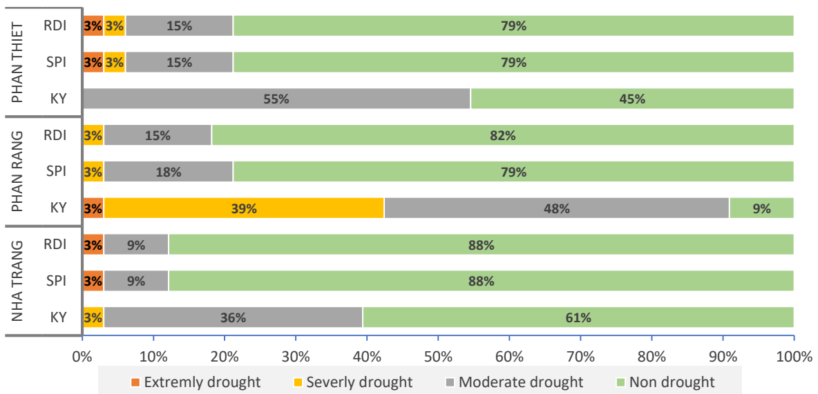
Figure 3. Comparison of percentage of drought severity categories identified
