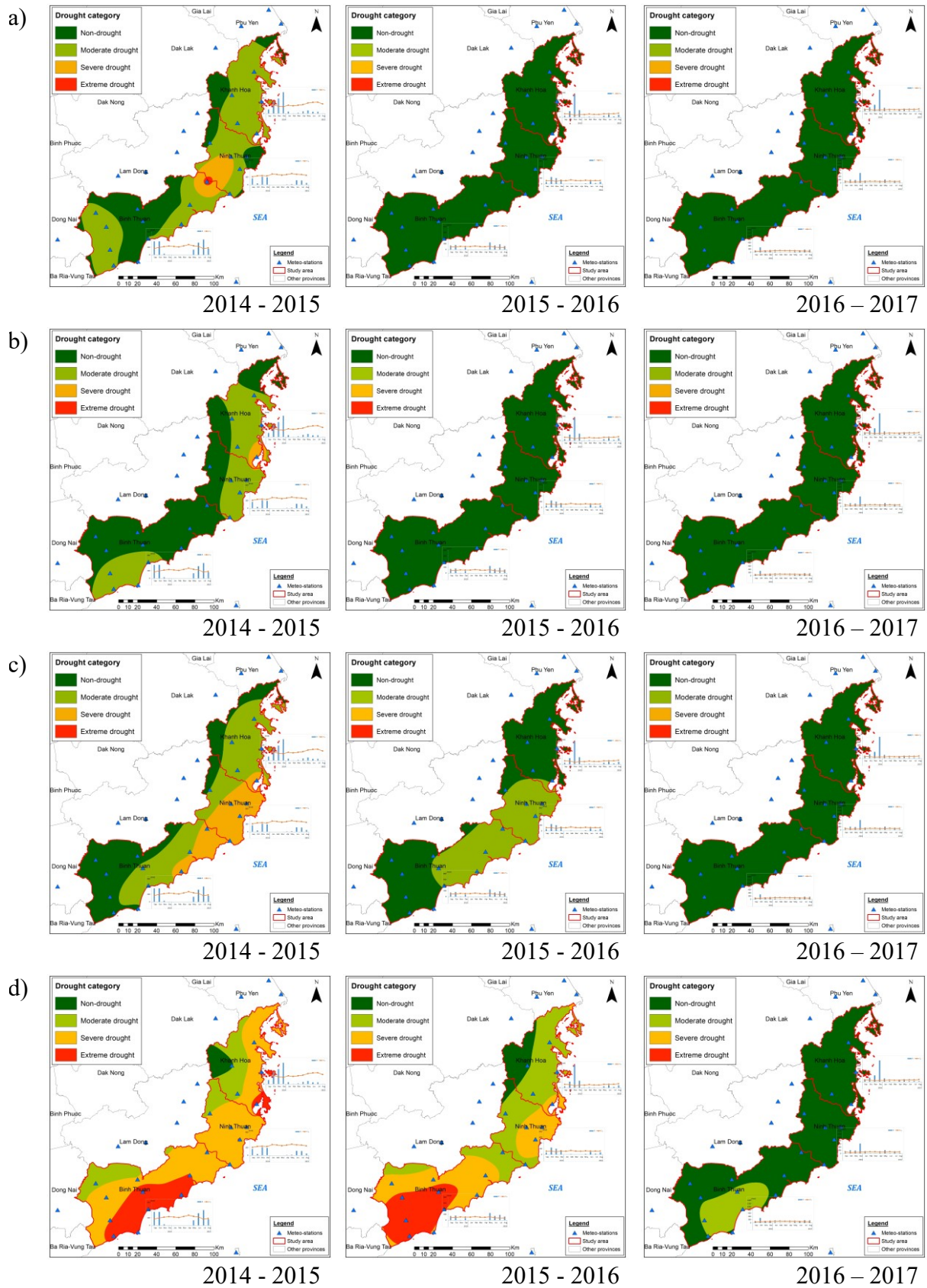
Figure 4. Spatial distribution of drought using different methods: (a) SPI, (b) RDI, (c) K_y , and (d) K_{y(w)} in hydrological year 2014-2015, 2015-2016 and 2016-2017
